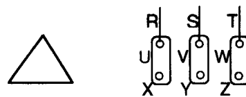
Delta connection D
